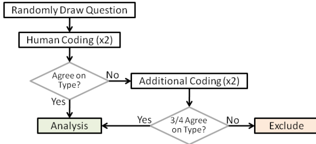
Figure 3. A flowchart showing how a randomly drawn question was classified by two or more coders.
